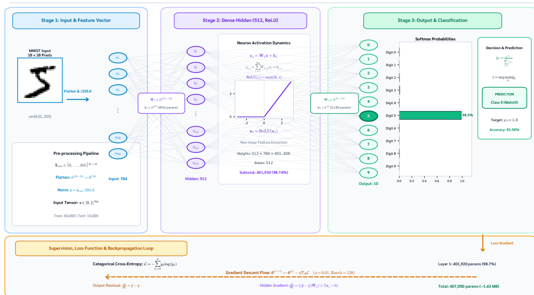
Figure 2: System Architecture & Computational Dataflow (Baseline 784-512-10 DNN)
